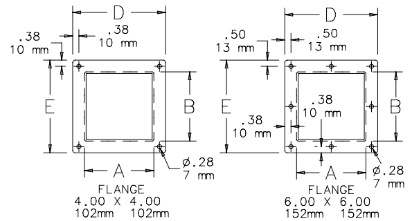
Flange Detail
