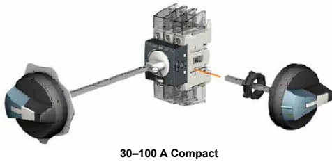
30–100 A Compact
