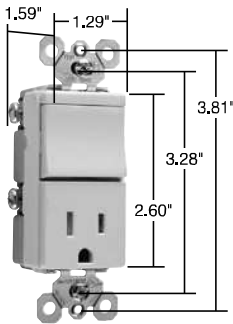
TM838TRLACC
