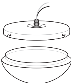
Figure 4 - Assembling the Globe
