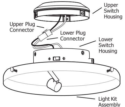
Figure 3 - Connecting the Plug Connectors
