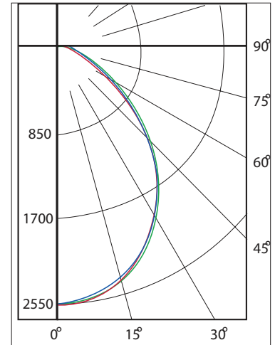
0° — 45° — 90° Candela Plot 2Lamp T8
