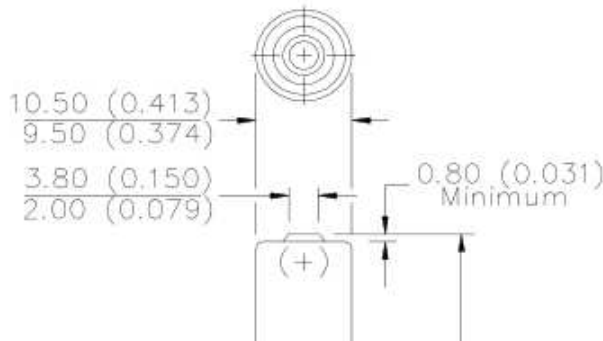
Industry Standard Dimensions in mm (inches)
