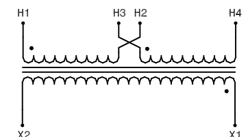
DUAL PRIMARY
