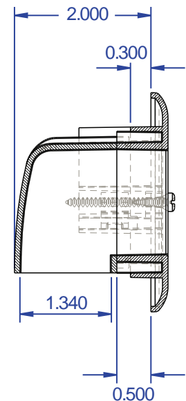
Side View 45-0008
