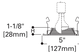
ERT401WHT High Gloss Appliance White Trim Ring with White Baffle
