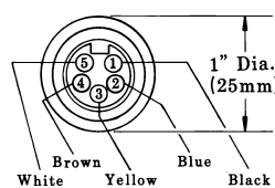
Cable Connector End View
