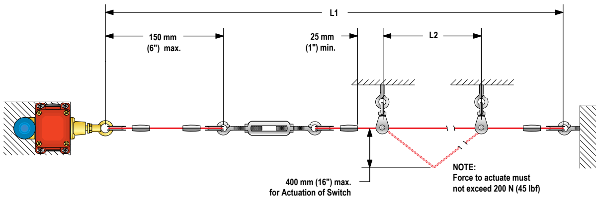
Figure 2. Assembly of Rope and Hardware
