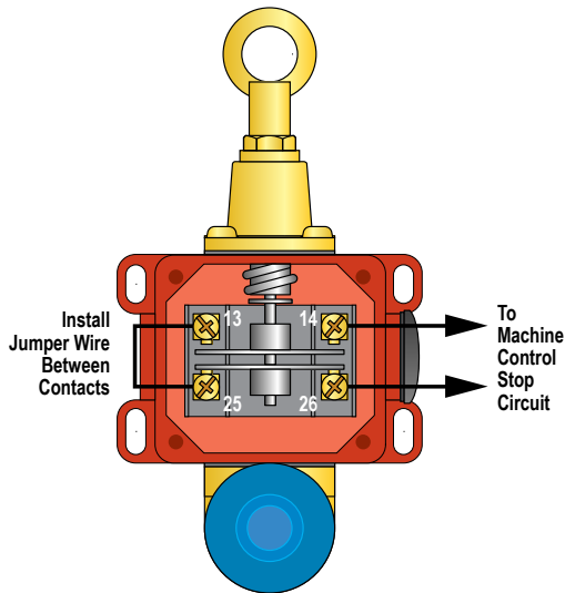
Figure 6. Wire the two switch contacts in series
