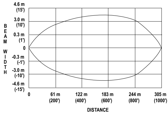
Figure 2. Beam Pattern
