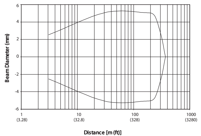
Beam Pattern—Transmitted Beam (300 m)
