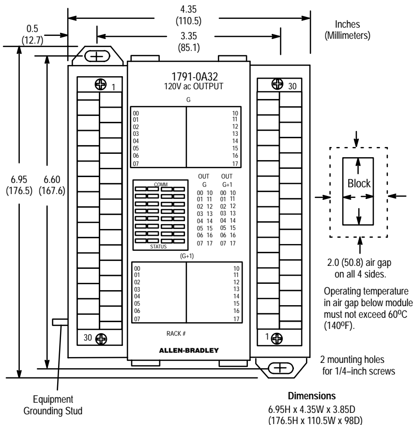
Figure 1 Mounting Dimensions for the Block I/O Module Cat. No. 1791-0A32 (PLC version shown)
