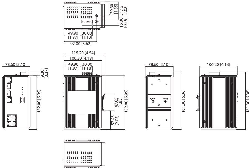
Panel Cut-out Dimensions: 115.2 x 152 x 78.6 mm (4.54" x 5.99" x 3.1")
